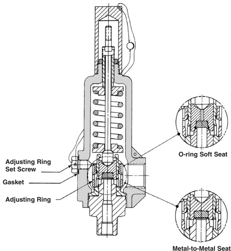
Series 800 Adjustable Blowdown Pressure Relief Valve
