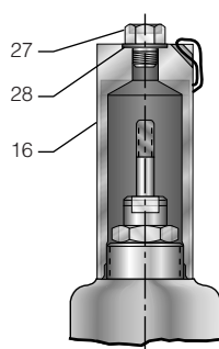
Type B Threaded Cap with Test Rod
