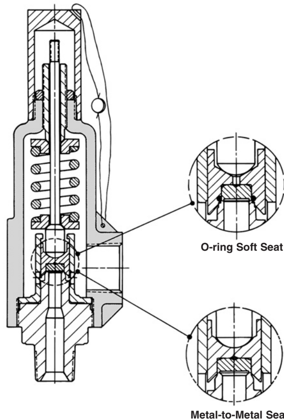
Series 900 Fixed Blowdown OMNI-TRIM® Pressure Relief Valve
