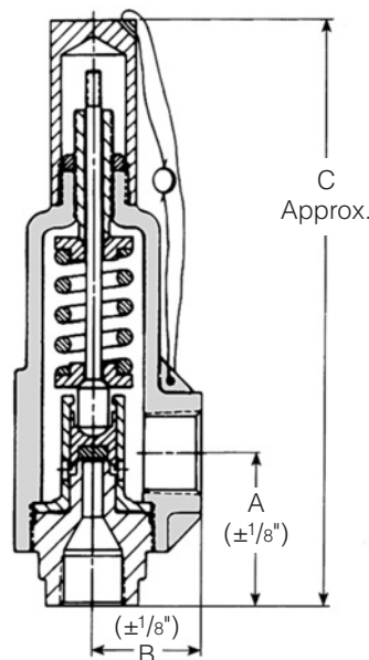
FNPT x FNPT
