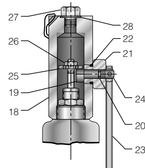
Type E Packed Lifting Lever with Test Rod
