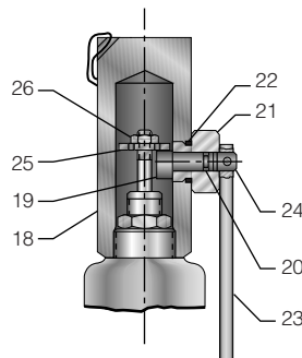
Type D Packed Lifting Lever
