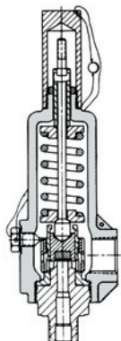
Standard Threaded MNPT x FNPT¹
