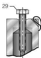
View Showing Valve Gagged Types B and E with Test Rod
