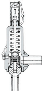
Male SW x Male SW⁵ (Socket Weld)
